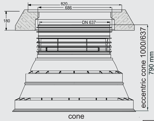
Cone (i) 1000/637 Eccentric cone height: 280-580 mm
