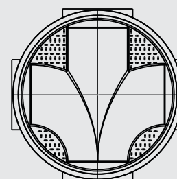
Cross line base ID-OD corrugate or smooth wall connection
